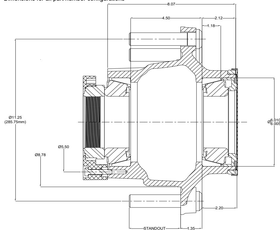
Dimensions for all part number configurations
